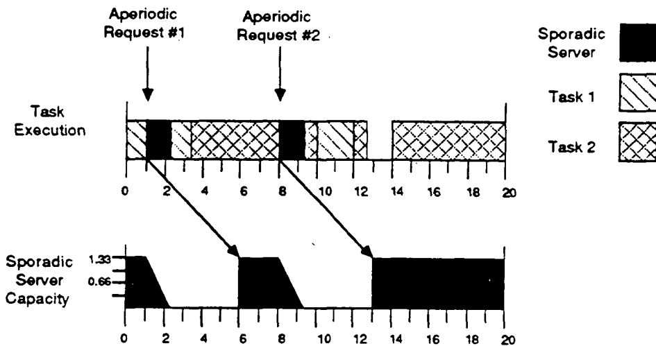
Figure 3-3: High Priority Sporadic Server Example
