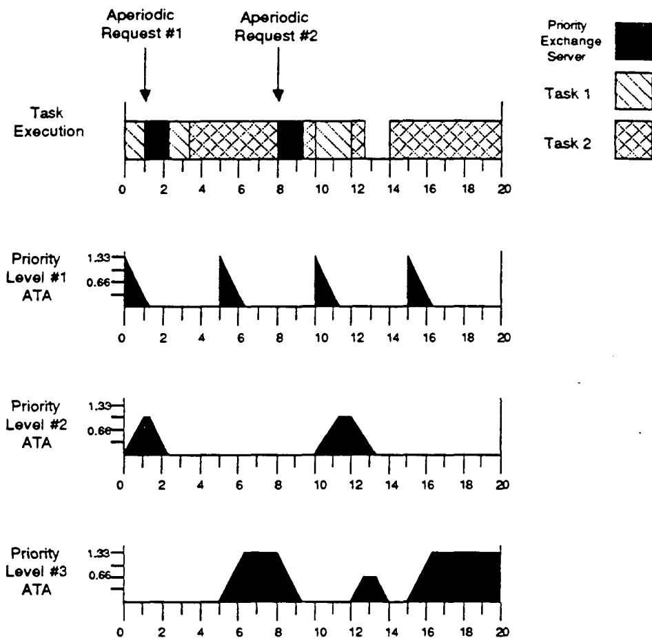
Figure 3-2: Priority Exchange Example
