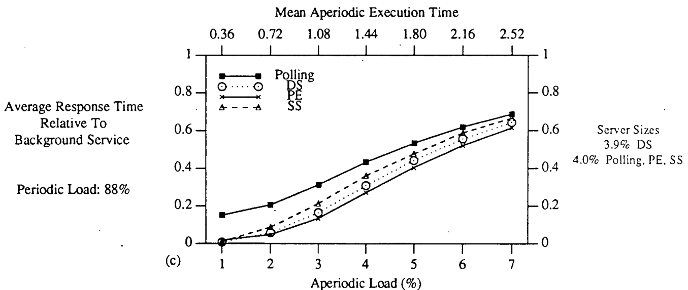
Figure 3-11: SS Algorithm Performance Comparison, Mean Aperiodic Interarrival Time = 36
