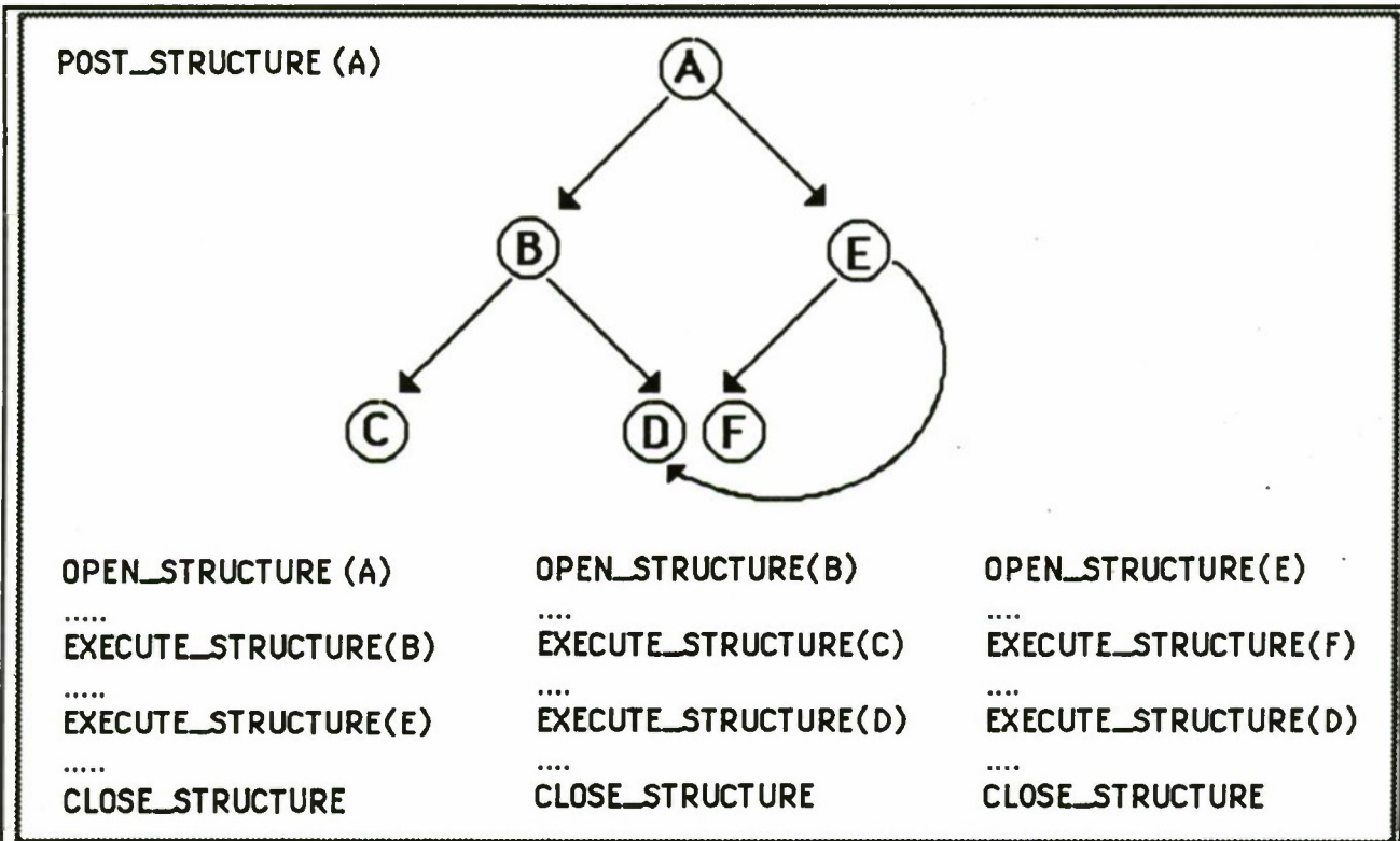
Figure 5.9: A PHIGS STRUCTURE is an oriented acyclic graph.
