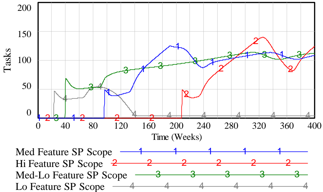
Figure 11: Simulation Results for Production Development Discovered Quality Issues
