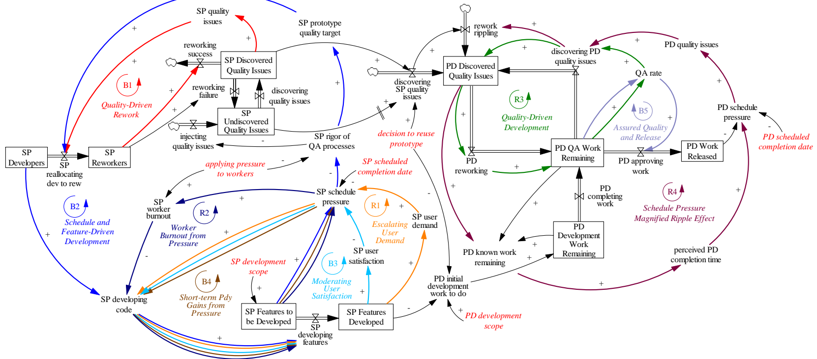
Figure 5: Overview of the System Dynamics Model
