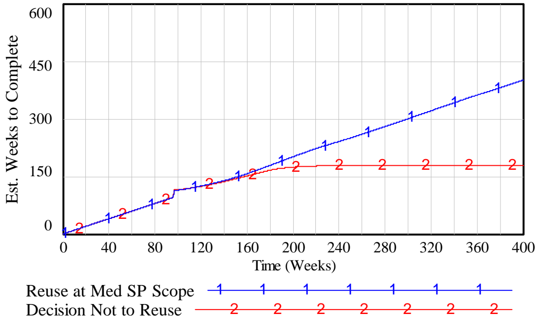
Figure 12: Simulation Results for Production Development Scheduled Completion Date Reflecting the Decision to Reuse
