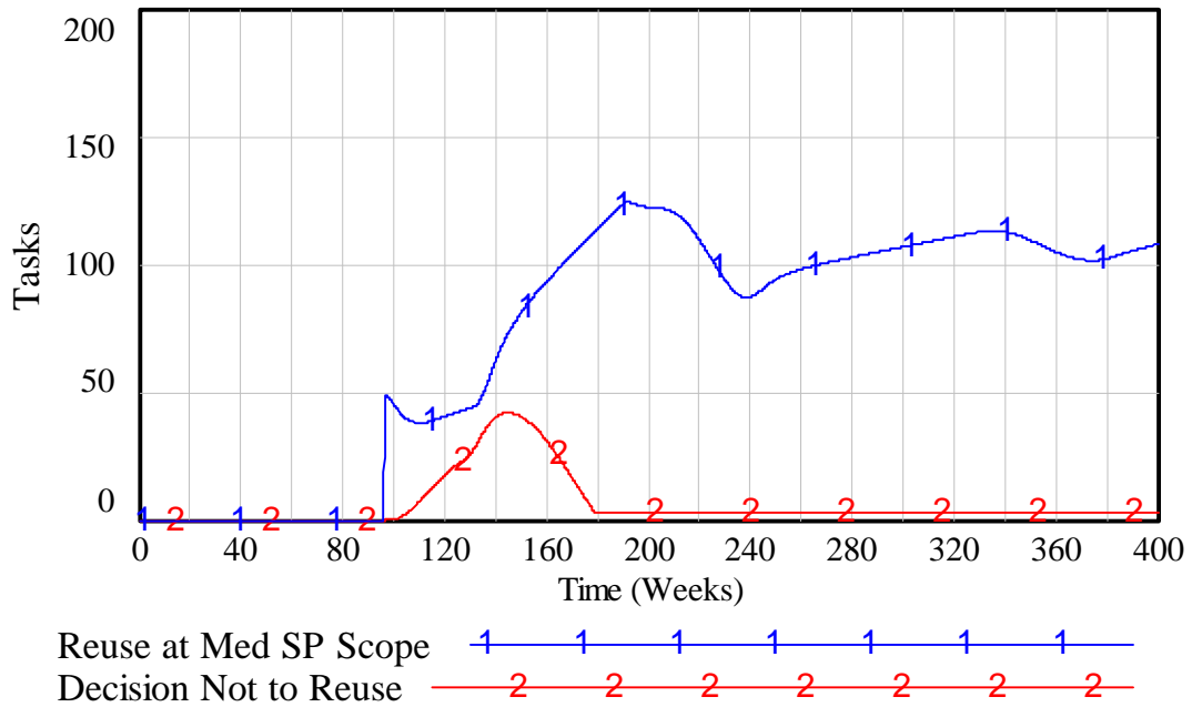
Figure 13: Simulation Results for Production Development Discovered Quality Issues Reflecting the Decision to Reuse
