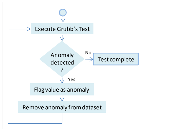
Figure 6: Grubbs' Test Algorithm
