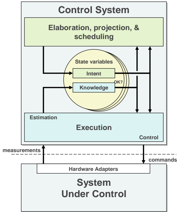
Figure 2: MDS Architectural Separation of Concerns [Bennett 2006]
