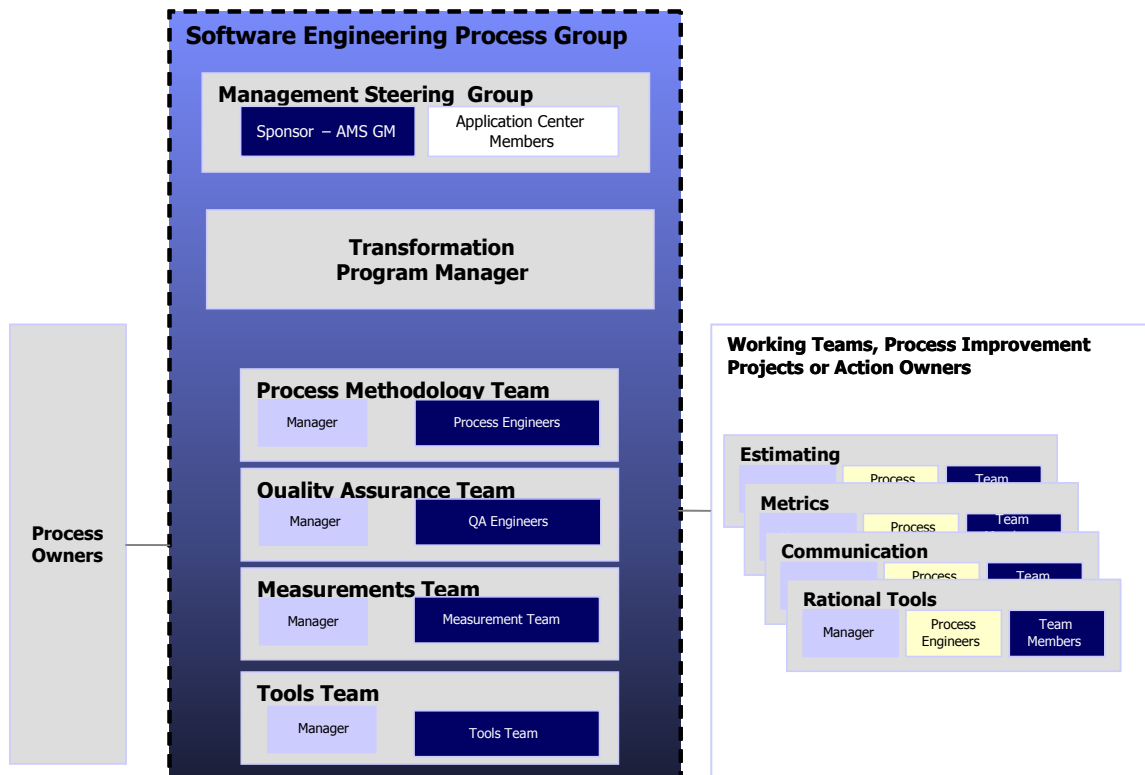
Figure 15: SEPG Structure
