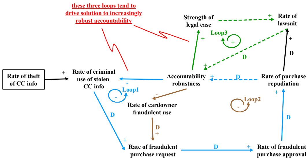
Figure 20: Composing Influence Diagrams of the First Iteration
