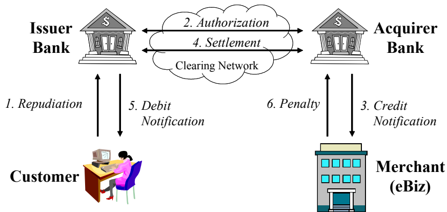
Figure 17: Online Credit Card Payment Repudiation
