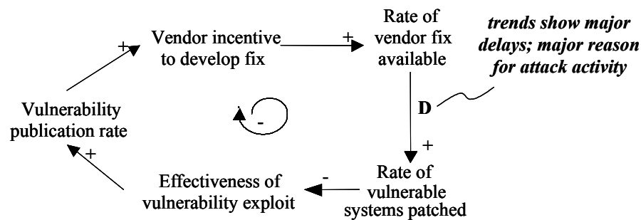
Figure 12: A Feedback Loop for Controlling Vulnerability
