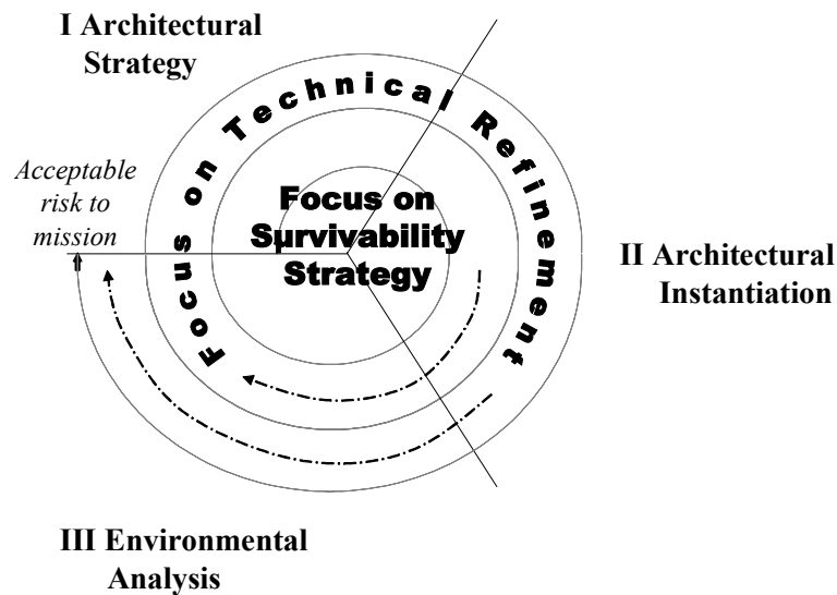
Figure 3: Execution of TRIAD
