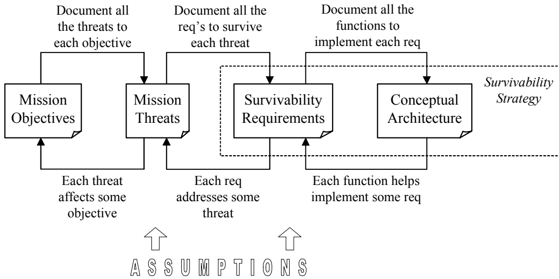
Figure 8: Survivability Tracing from Mission to Conceptual Architecture
