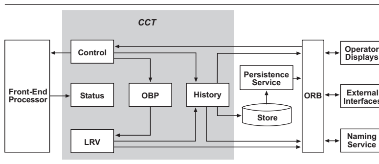
Figure 2: CCT Execution Architecture: Data Flow View
