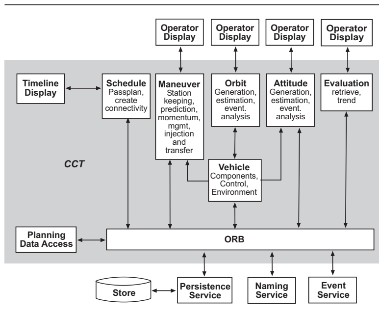
Figure 3: CCT Planning Architecture: Data Flow View
