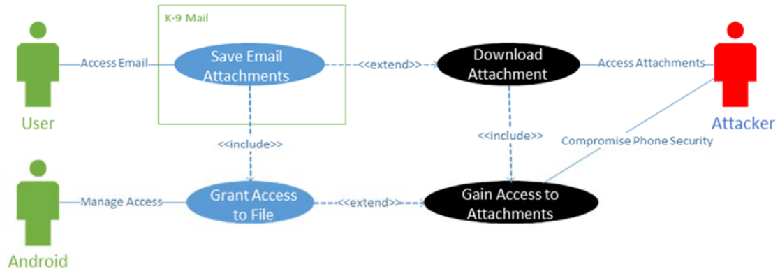
Figure 15: Misuse Case MUC4
