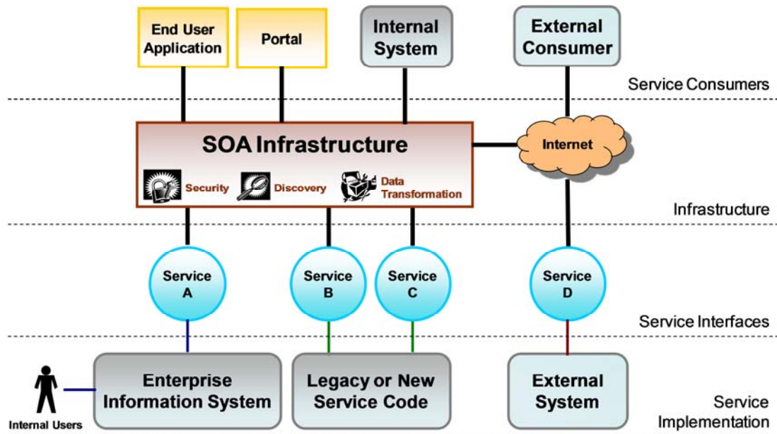
Figure 1: High-Level Notional View of a Service-Oriented System
