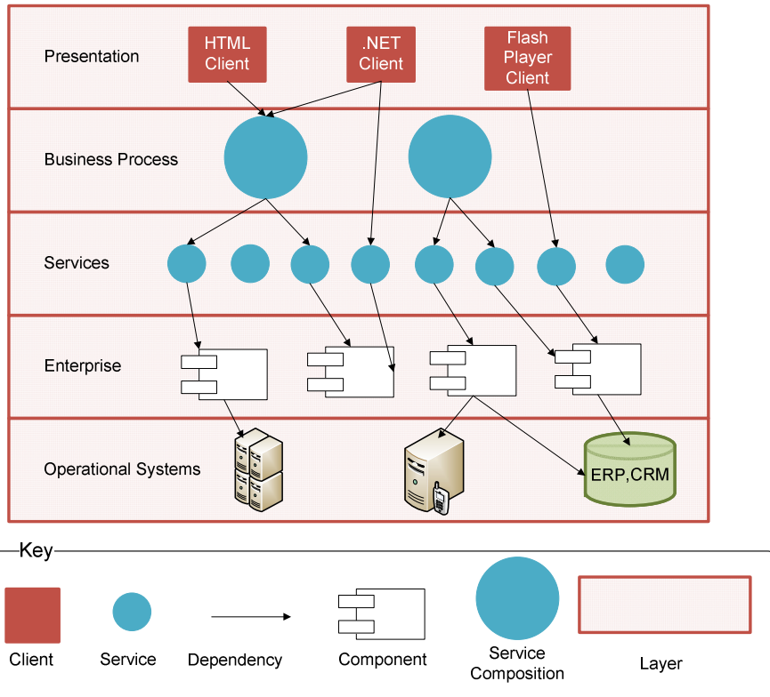
Figure 1: SOA Layers
