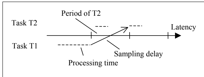
Figure 6: Asynchronous Sampling
