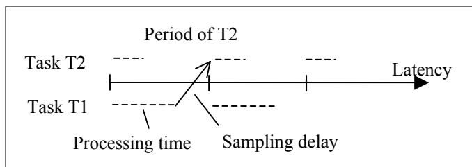
Figure 7: Synchronous Sampling
