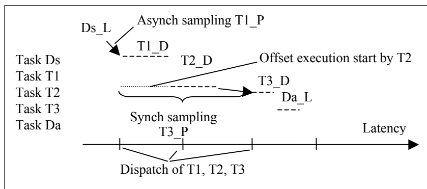
Figure 14: The Effect on Latency of Mixing Immediate and Delayed Data Port Connections
