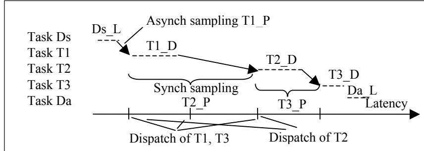
Figure 13: Harmonic Sampling
