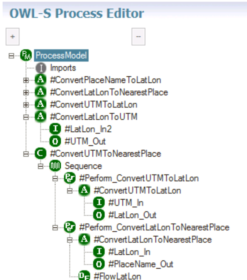
Figure 10: Simple and Composite Services Represented in the OWL-S Process Editor
