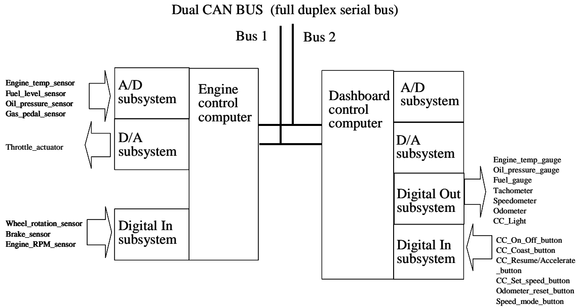
Figure 5: Dashboard/Cruise Control Hardware Architecture
