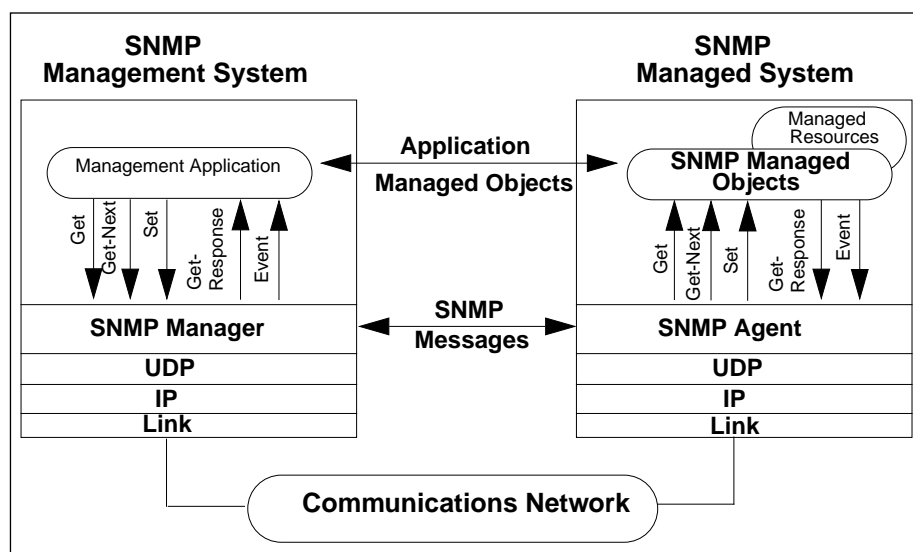
Figure 25: The SNMPv1 Architecture [Lake 96]
