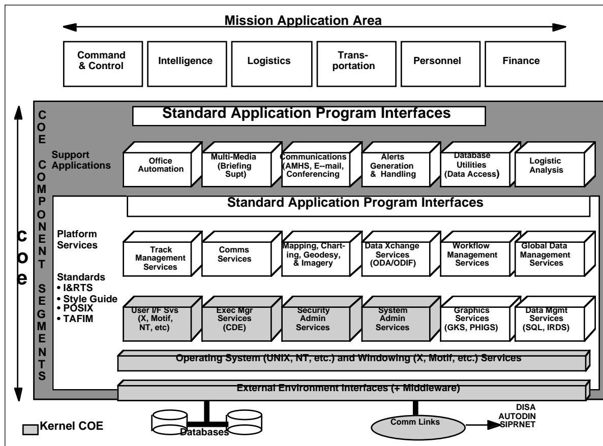
Figure 9: Defense Information Infrastructure Common Operating Environment [DII COE 96]
