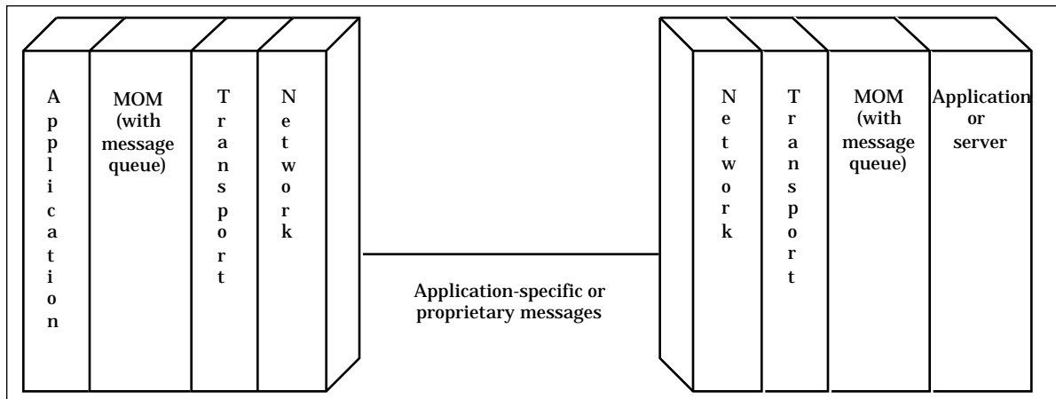
Figure 16: Message-Oriented Middleware
