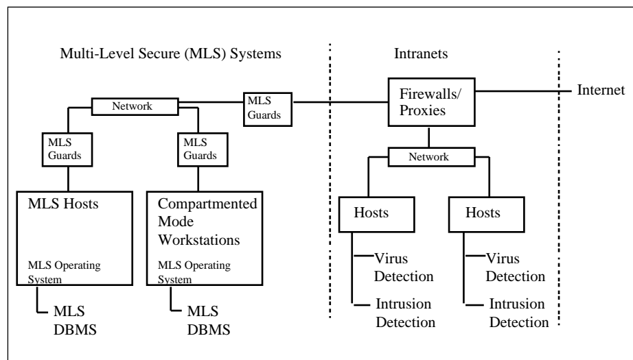
Figure 5: Computer System Security in C4I Systems
