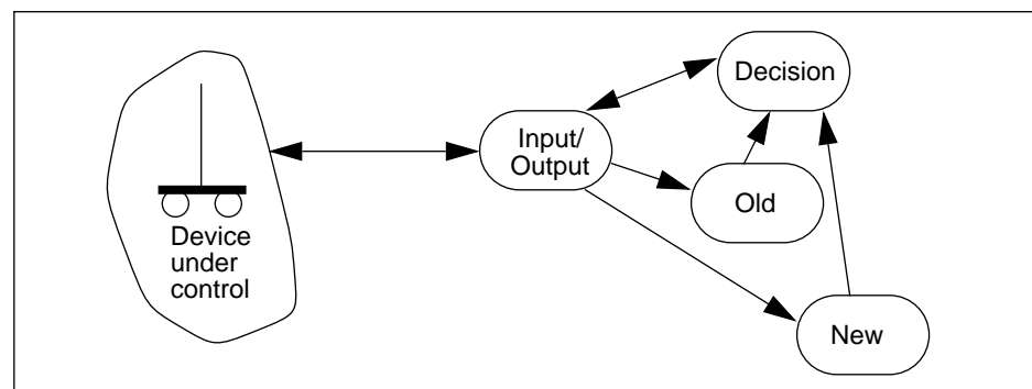
Figure 26: Simplex Architecture: Simplified Data Flow
