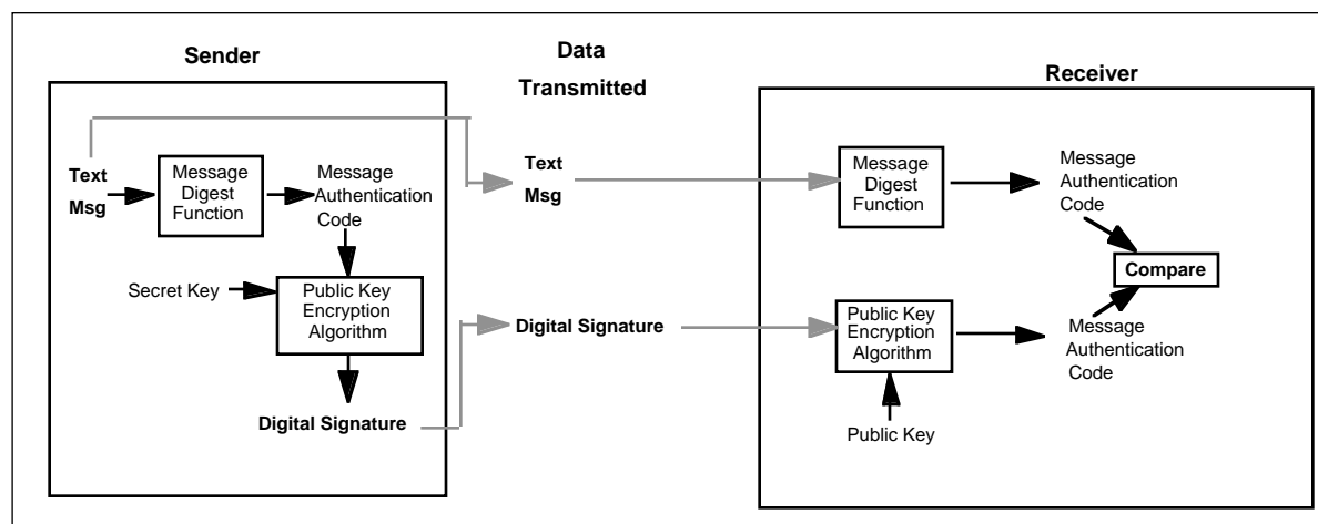
Figure 22: Public Key Digital Signatures
