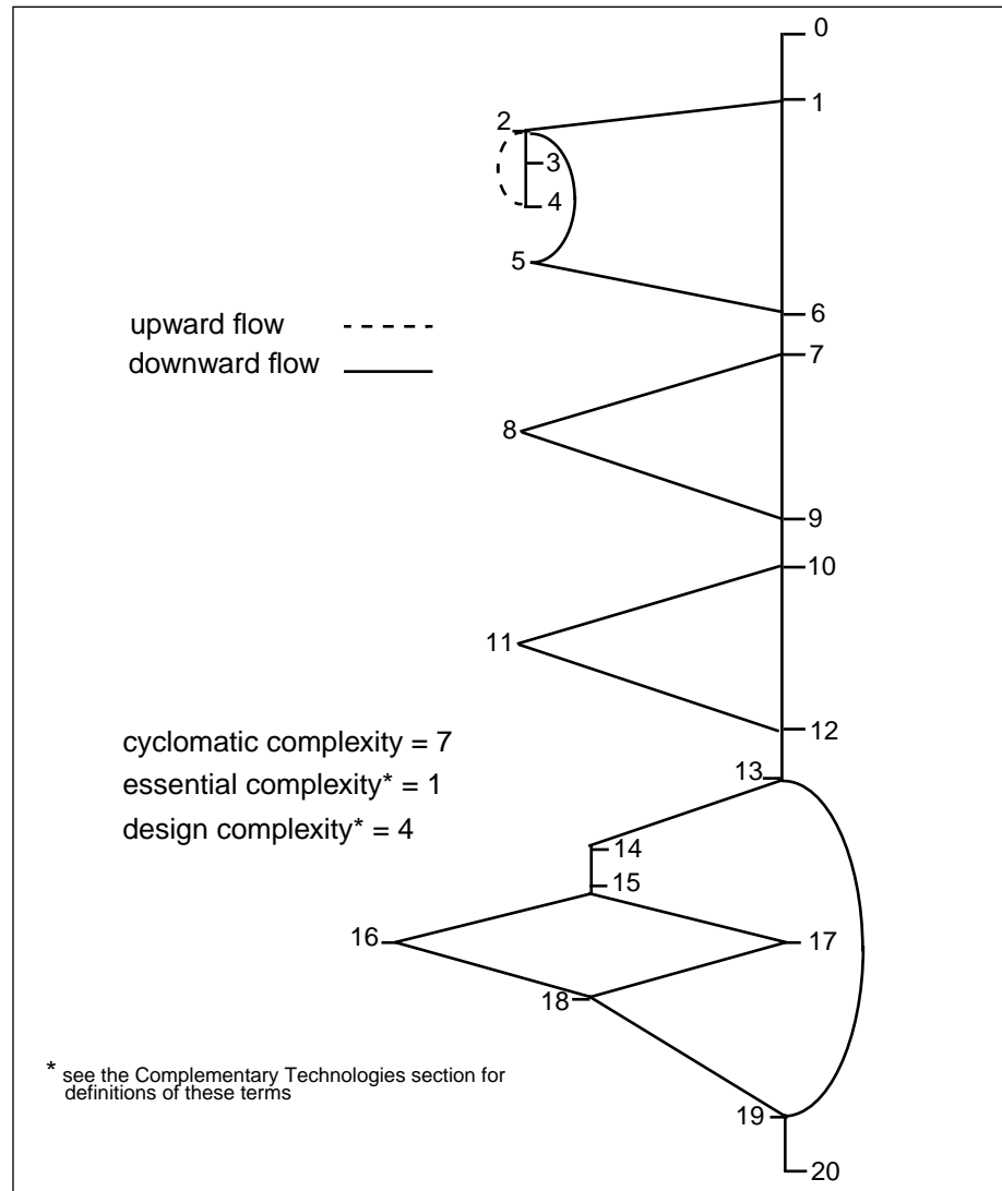
Figure 6: Connected Graph of a Simple Program
