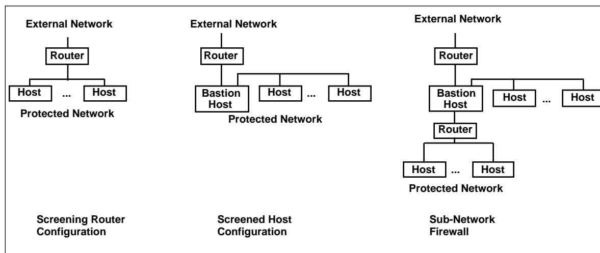
Figure 13: Firewall Configurations
