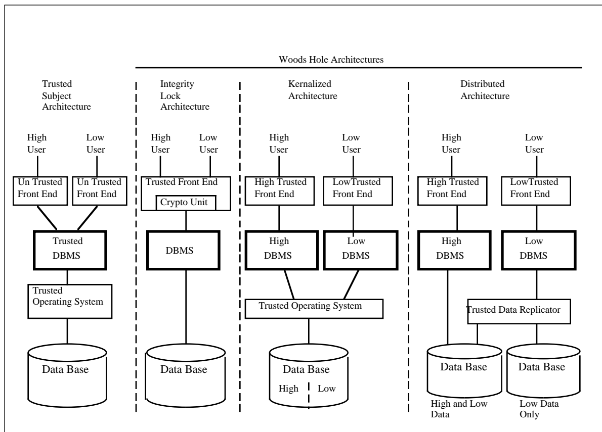
Figure 20: MLS DBMS Schemes
