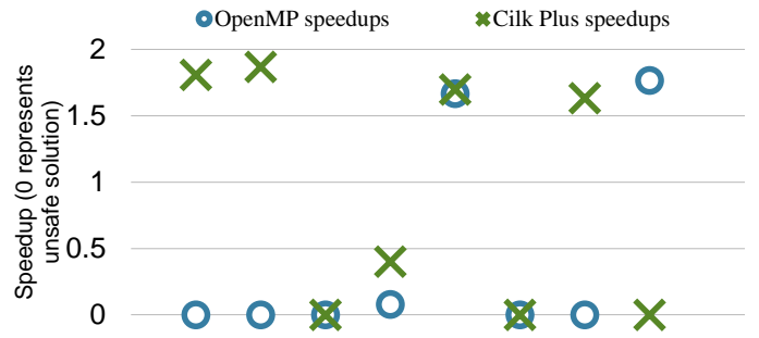
Fig. 1. Speedups by parallel language extension.
