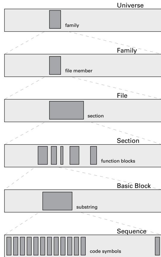
Figure 1: Organization and grouping of static features in software corpora
