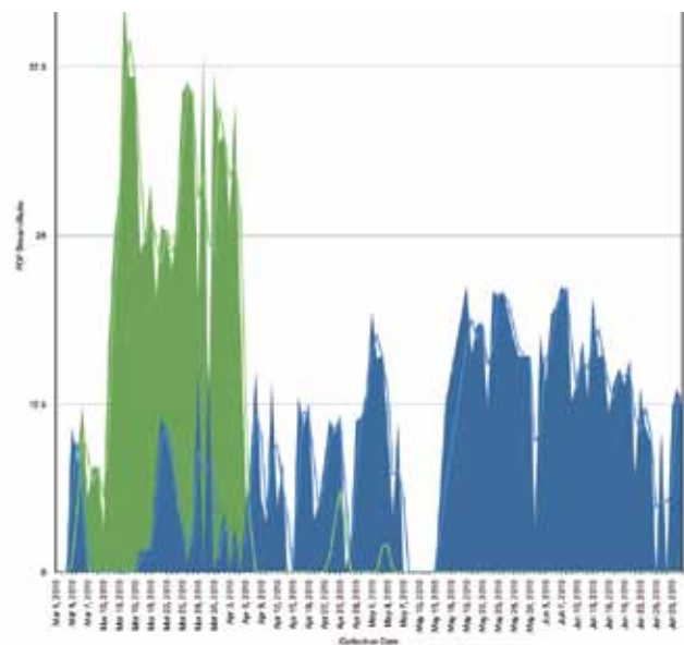
Figure 1: Ratio of collected getAnnots() stream obfuscation objects
