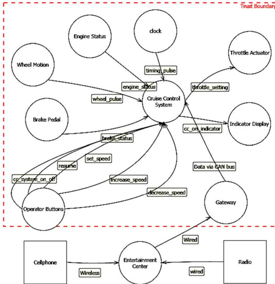
Figure 8: Trust Boundary for CAN Bus
