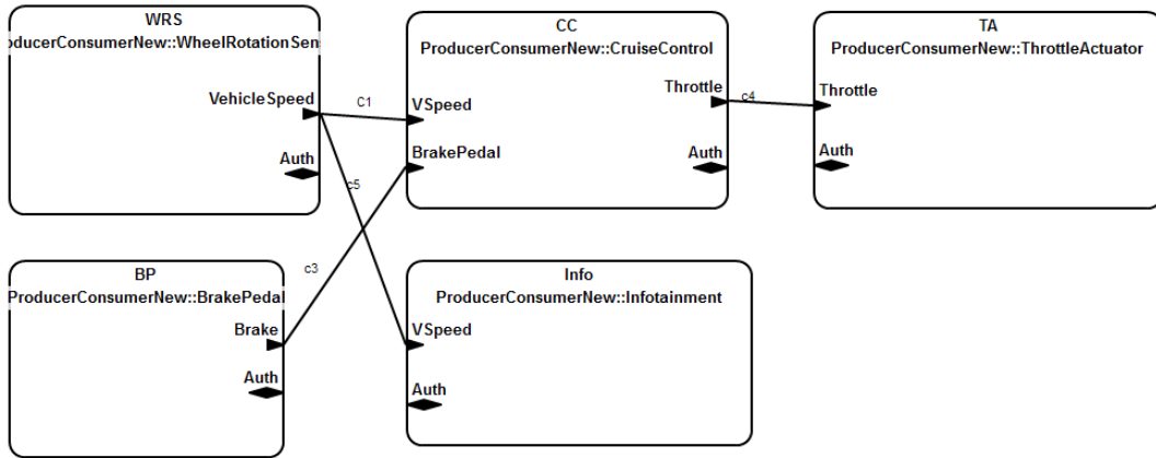
Figure 12: Component and Connector View of a Subset of the Model Problem
