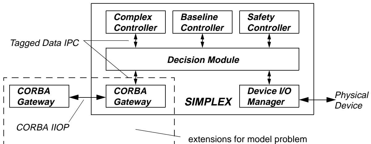
Figure 3-2: Extending Simplex with CORBA Gateways
