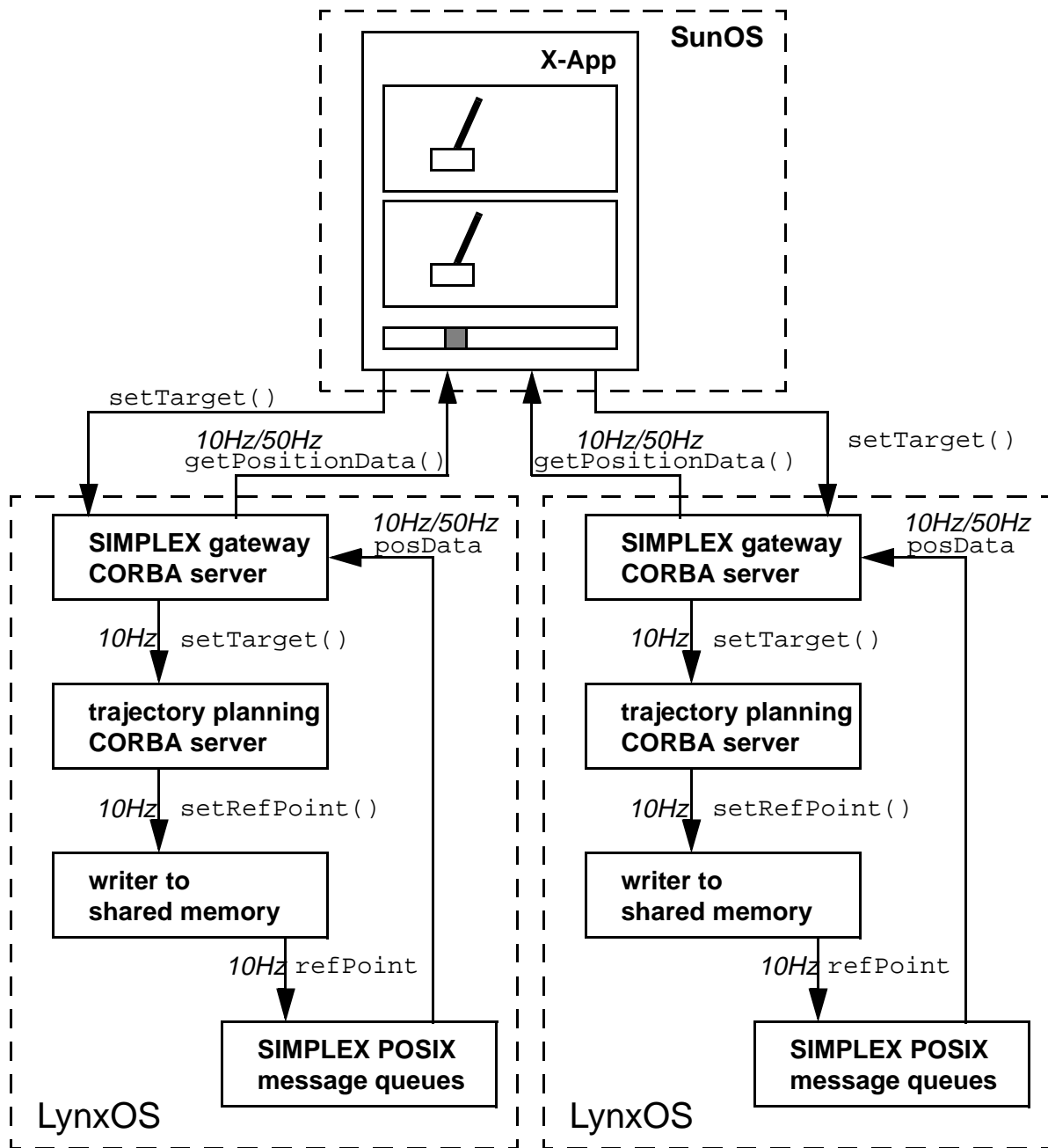
Figure 3-4: Communication Structure for the Synchronized Inverted Pendulum
