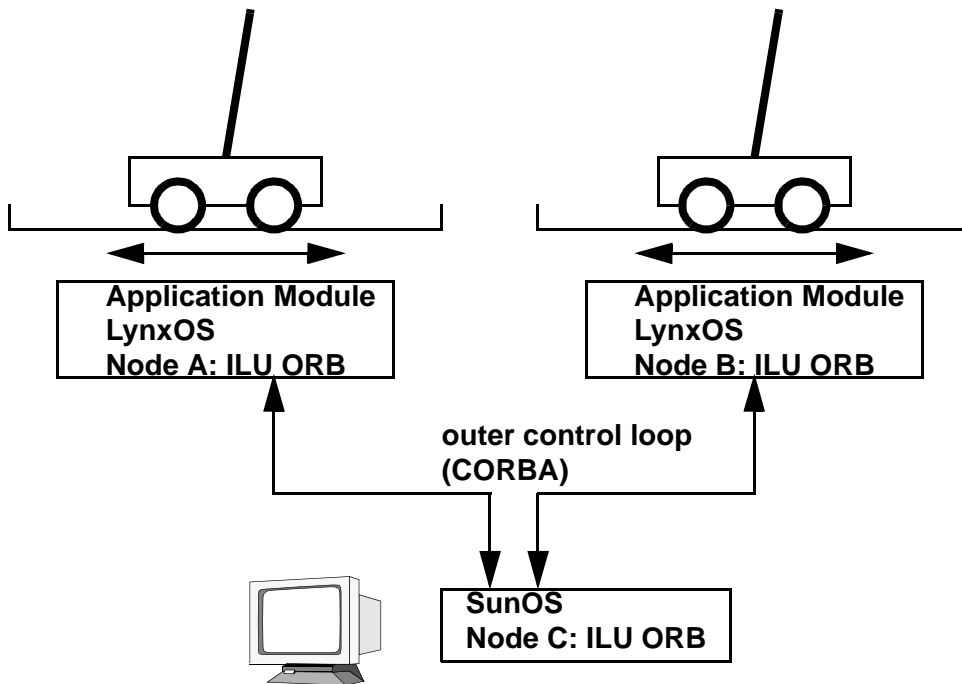
Figure 3-1: Synchronized Inverted Pendulum Scenario
