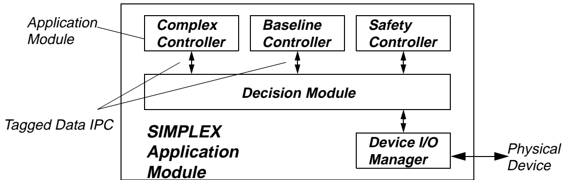
Figure 2-1: Simplex Architecture
