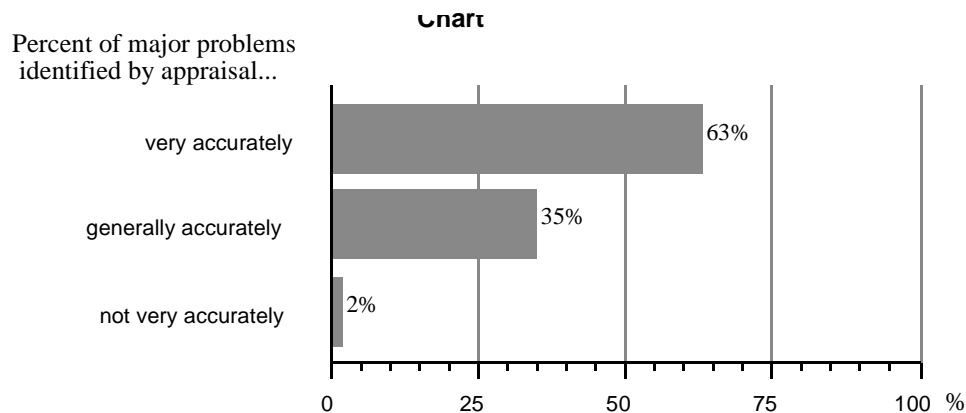
Figure 4-1: Accuracy in Identifying Major Software Problems
