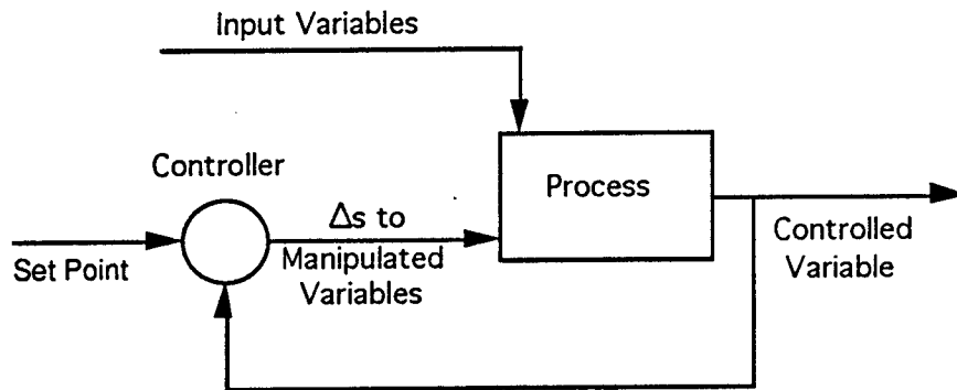
Figure 3: Feedback Control
