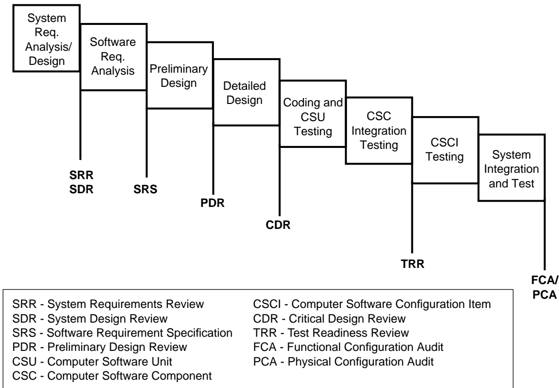
Figure 1-5 DoD-STD-2167A Activities
